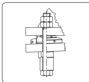
Spherical washer
