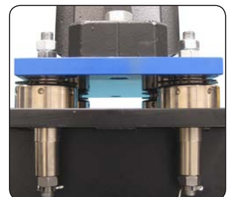
Extended SKF Vibracon chock
